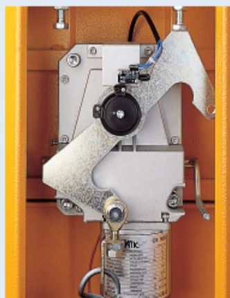
Manual release device
